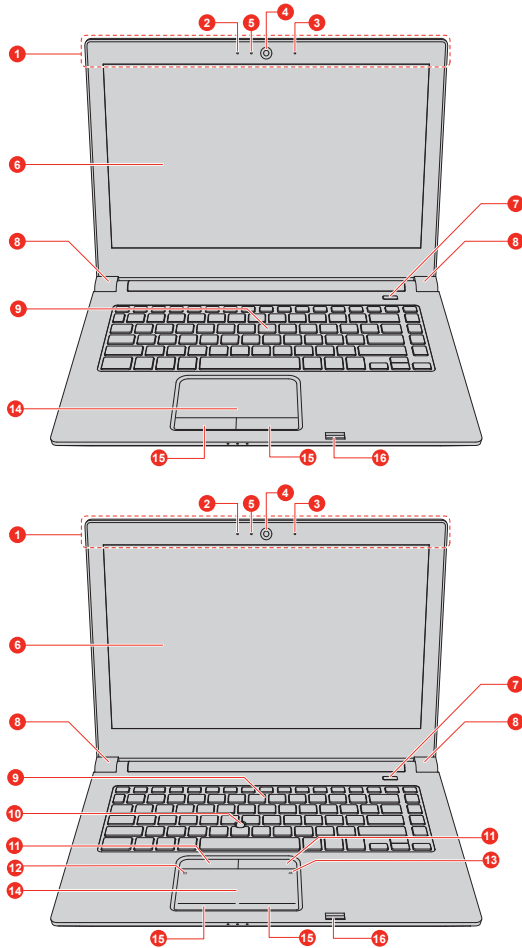
Figure 3-12 The front of the computer with the display panel open (A40-D)
