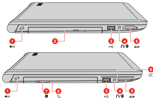
Figure 3-8 The left side of the computer (A40-D)
