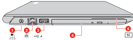
Figure 3-2 The left side of the computer (A30-D)
