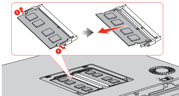
Figure 4-14 Removing the memory module
