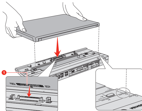
Figure 4-23 Aligning your computer with the Port Replicator (A40-D)
