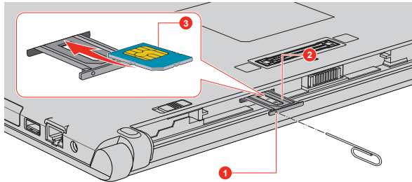
Figure 4-8 Open the SIM card tray with the eject hole (A30-D)
