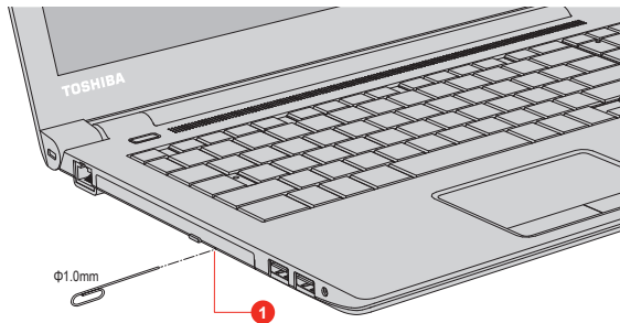
Figure 4-4 Manual release with the eject hole
