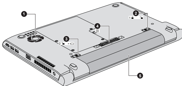
Figure 3-5 The underside of the computer
