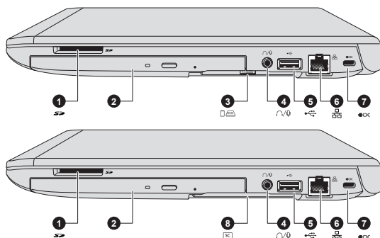
Figure 3-3 The right side of the computer
