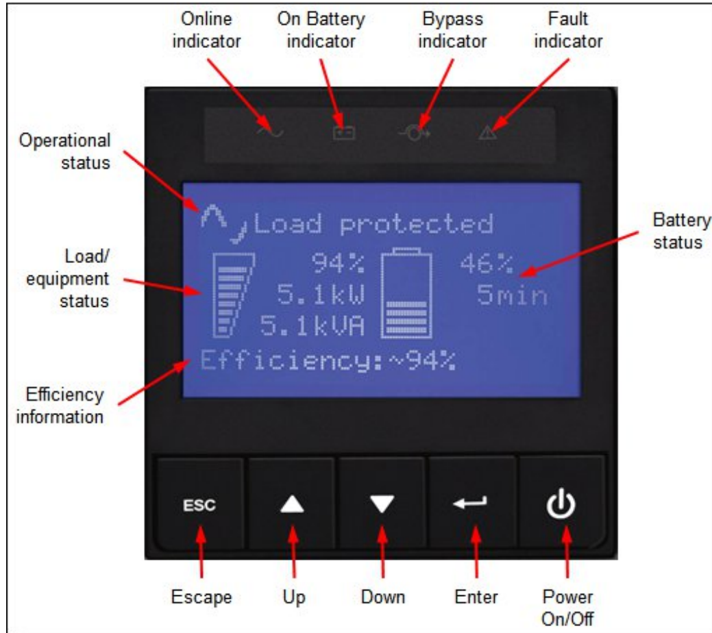
Figure 4. Control panel on the front of the RT5kVA or RT6kVA 3U Rack or Tower UPS
