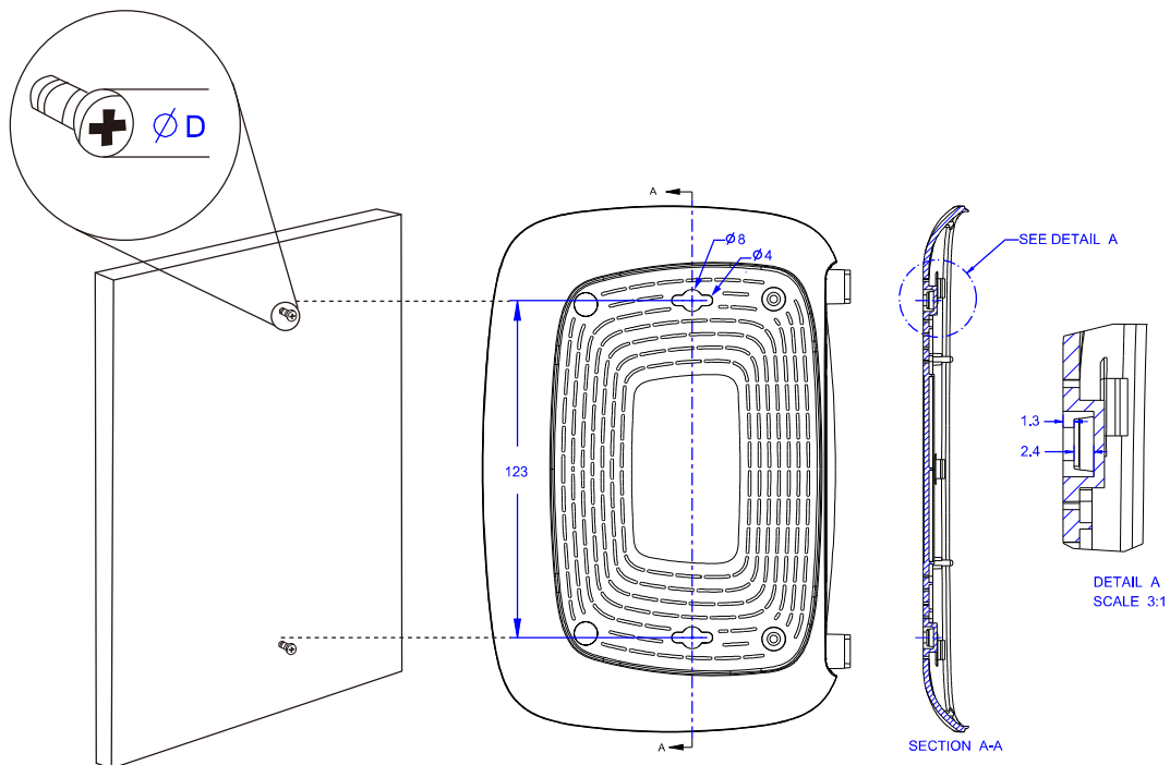
Figure 2-2 Wall-mount Install
